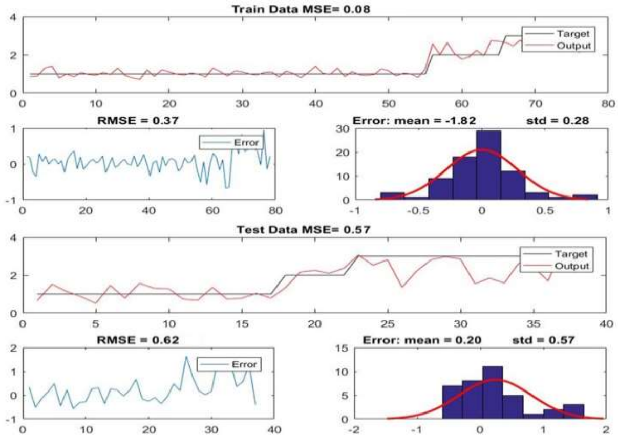
Figure. 8 Train and test errors for our dataset (DE learning)
