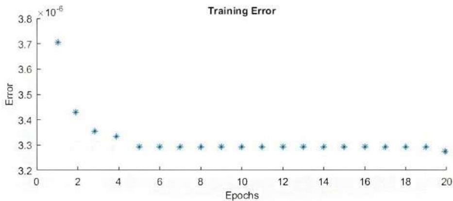
Figure. 5 Training FIS using hybrid learning in 20 epoch
